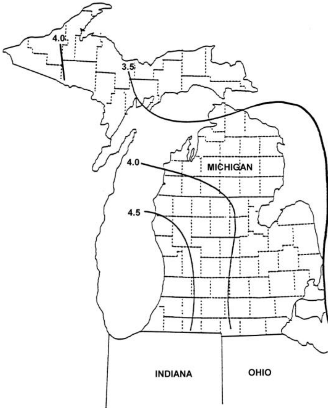
Figure B.4 - 25-year, 24-hour Rainfall
